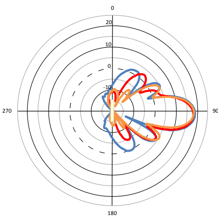
H-pol Elevation
